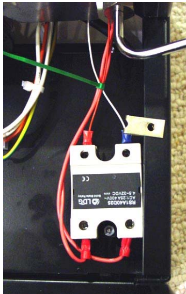
Figure 10. SSR installed.
